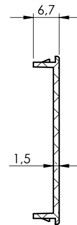
SECTION B-B
